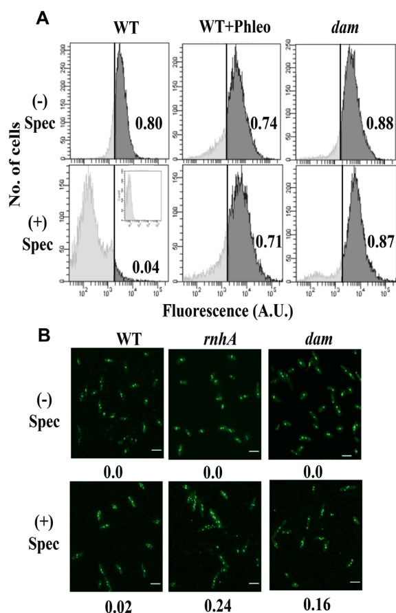
Figure 1. cSDR in dam mutants. (A) Analysis by flow cytometry, as described (52), of DNA synthesis in cultures of (i) parental (WT) strain GJ18609, (ii) WT with phleomycin (WT+Phleo) at 1 \mu g/ml, and (iii) the isogenic dam mutant GJ16494 ( dam ), without (–) or with (+) treatment with spectinomycin (Spec). In each panel, the proportion (of the total) of cells in which the fluorescence value exceeded the gating threshold (vertical line) is given at right. Inset within bottom left panel depicts fluorescence in cells exposed to neither EdU nor Alexa Fluor 488 (that is, autofluorescence). (B) Fluorescence microscopy for detection of ParB::YGF- parS foci in cells from cultures of plasmid pAD16-bearing derivatives of parental (WT) strain GJ15830 and its isogenic rnhA or dam mutants (GJ15831 and GJ15832, respectively) without (–) or with (+) treatment with Spec. Beneath each panel, the proportion of cells with >2 foci is indicated (minimum of 300 cells examined). Scale bar, 3 \mu m.
